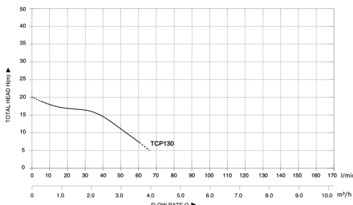
TCP 130 Centrifugal Pump
