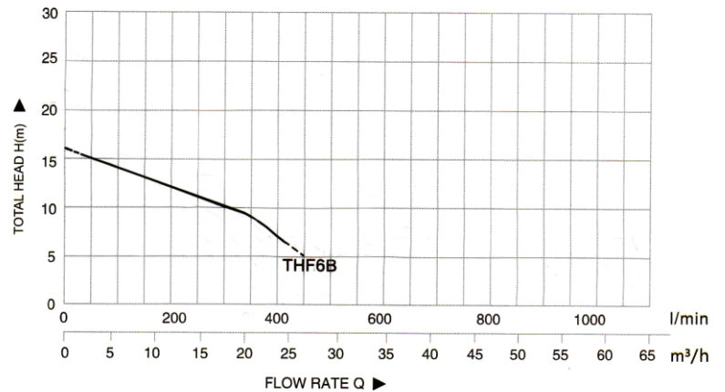
THF 6B Centrifugal Pump
