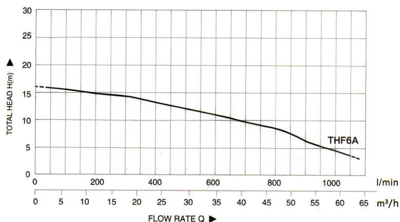
THF 6A Centrifugal Pump
